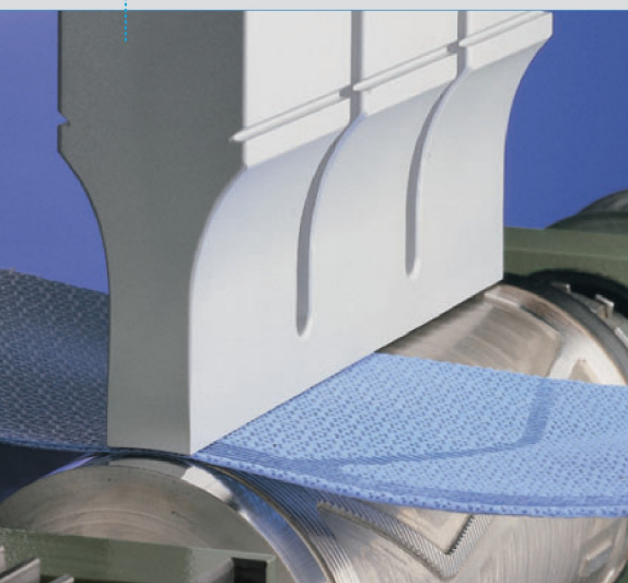
Ultrasonic welding system for the joining of multi-layer material
